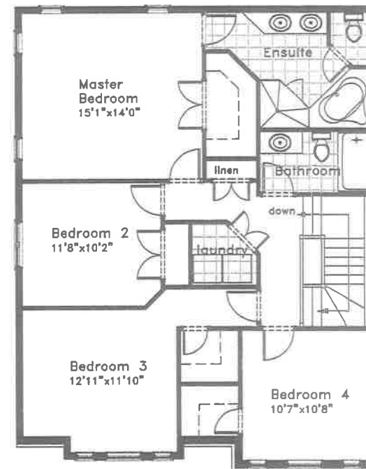
Second floor 1124 sq.ft.
