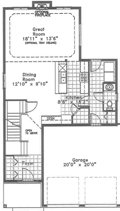
Ground floor 926 sq.ft.
